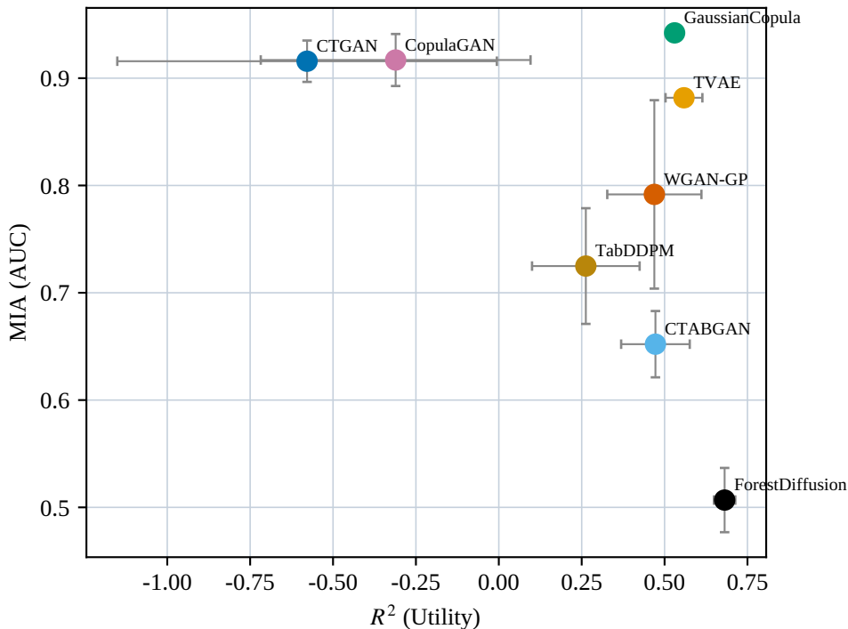
Real Estate: R^2 (Utility) vs MIA (AUC)
